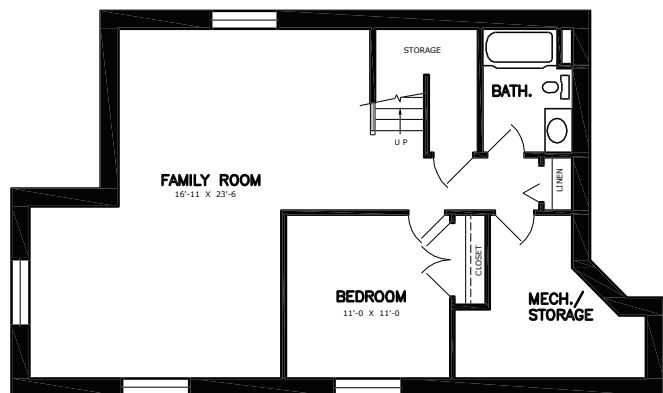
FINISHED BASEMENT
