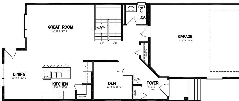
MAIN FLOOR
